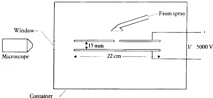
1.3 Millikan's experiment for the determination of the charge of the electron.
